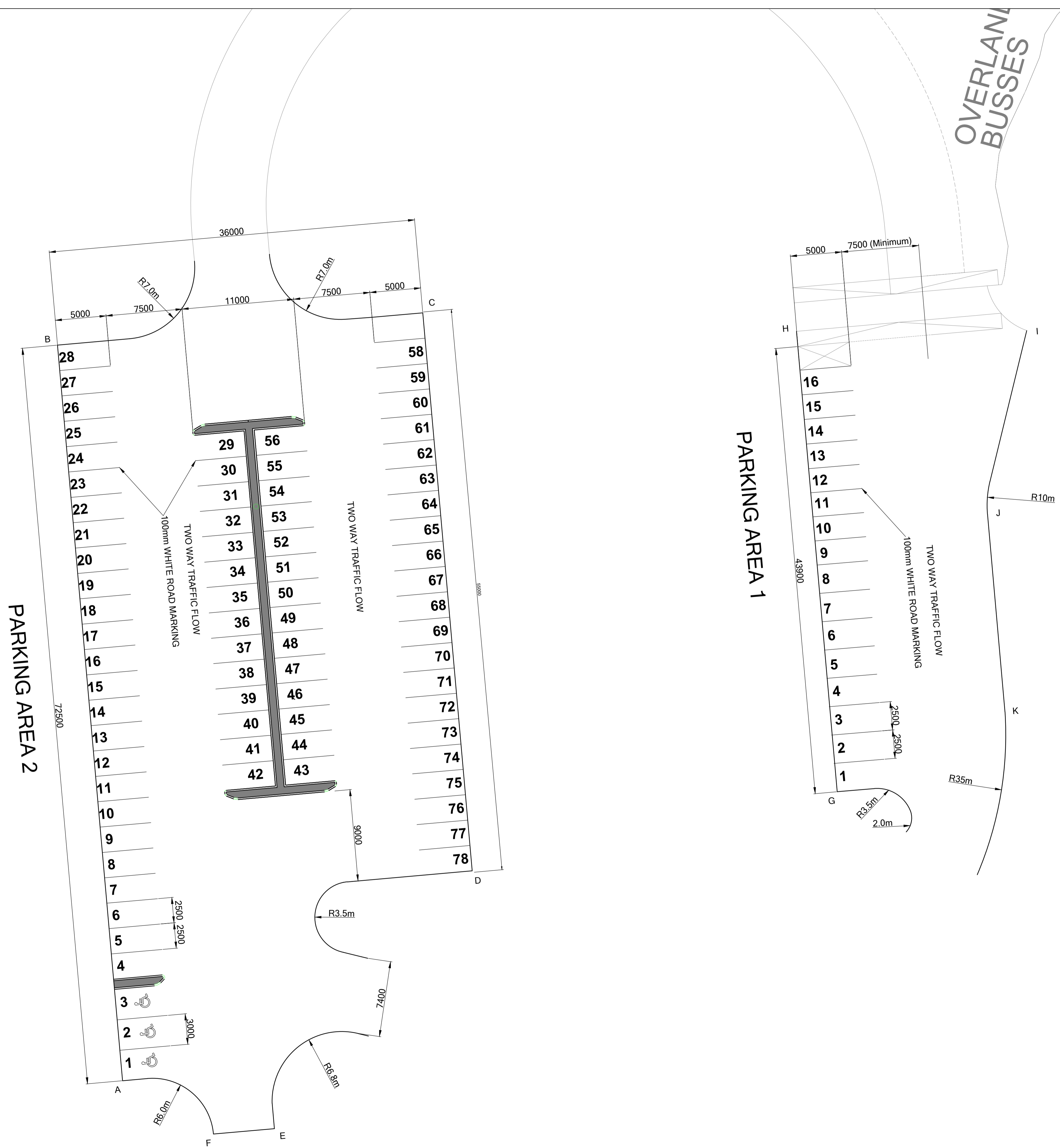
90° PARKING LAYOUT - BOTH SIDERS AND ONE SIDE OF ROAD
